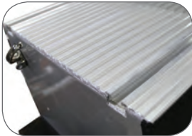
Side pack tops utilize the Stellar exclusive extruded aluminum top that has two accessory mounting rails to eliminate drilling and makes mounting and relocating accessories easy and secure.
